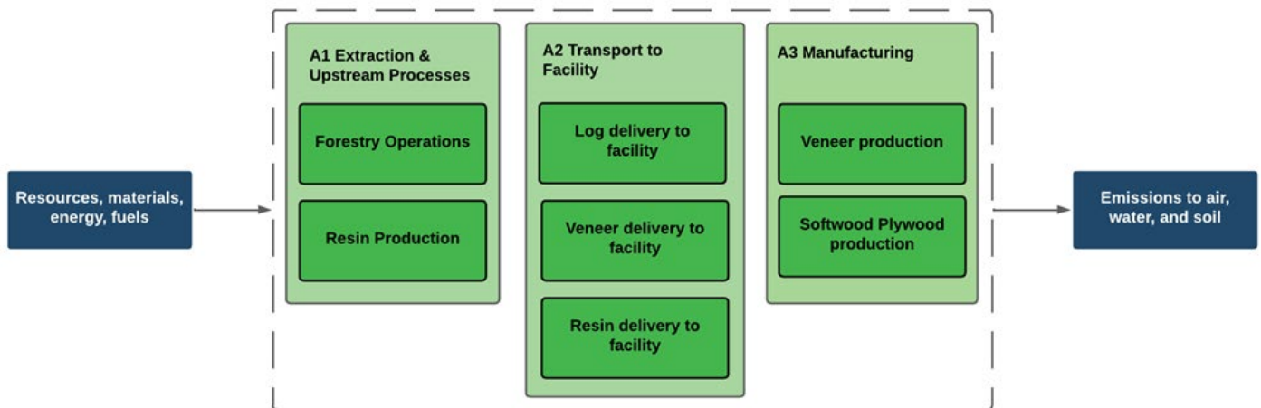
Figure 3. Cradle-to-Gate (A1-A3) System Boundary for Western Softwood Plywood Production.
