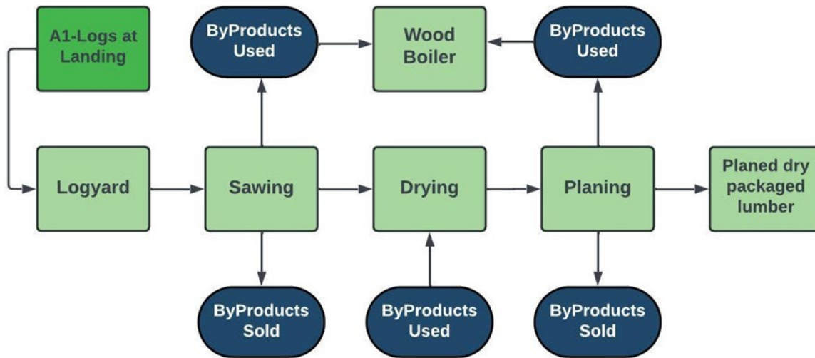
Figure 1. Sawmill Unit Processes from Roundwood to Planed Dry Lumber from Logs.
